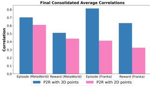
Figure 10. P2R Rank Order Correlations with 2D vs. 3D Points
