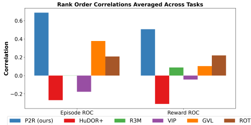
Figure 7. Metaworld Rank-Order Correlations with Camera Change (Robot Demo)
