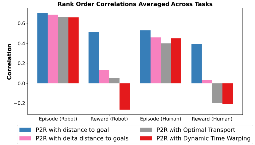
Figure 11. P2R Rank Order Correlations with Different Distance Functions in Meta-World
