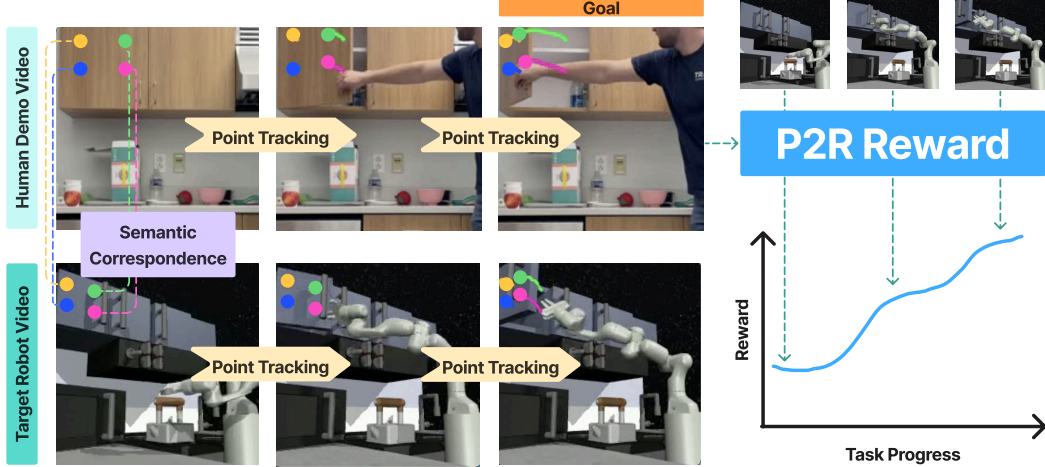
Figure 1. Overview of Points2Reward. We use semantic point correspondence and off-the-shelf point tracking to generate matching point tracks of the demonstration and rollout video. We then use the two point tracks to compute a goal-based reward.
