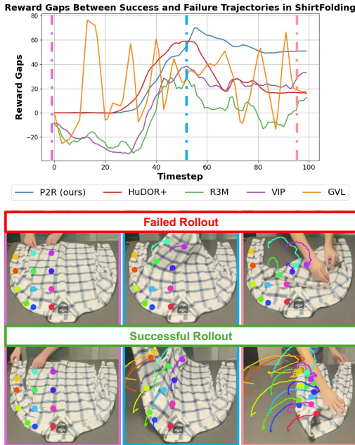
Figure 4. Reward gap between successful and failed shirt folding target robot videos. Colored points and lines on the shirt represent the initial point selections and their trajectories. Dashed lines on the plot correspond to the timesteps for frames that have the same color outline.
