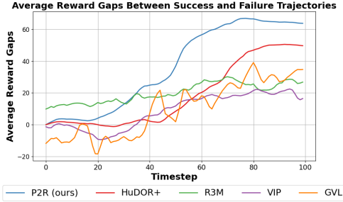
Figure 3. Instantaneous reward gap between successful and failed rollouts over time, averaged across 11 tasks (9 sim + 2 real world).
