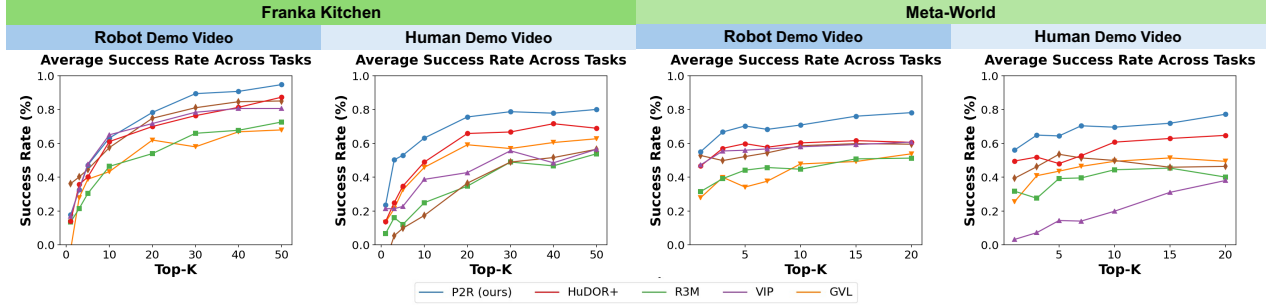
Figure 9. Behavior Cloning Performance Using Top k Robot Episodes from Mixed-Quality Datasets over varying k .
