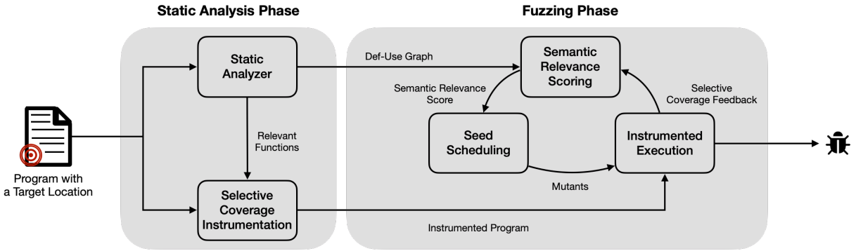
Figure 4: DAFL architecture.
