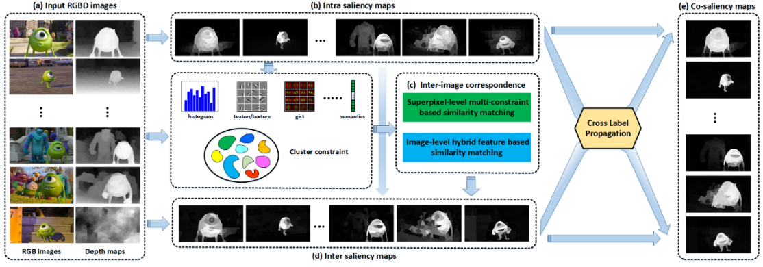
Fig. 4-1 Flowchart of the proposed RGBD co-saliency detection model. (a) The input RGBD images. (b) The intra saliency maps produced by existing single saliency method collaborating with depth information. (c) The inter-image correspondence is obtained by superpixel-level multi-constraint based similarity matching and image-level hybrid feature based similarity matching. Using the corresponding relationship and intra saliency maps, the inter saliency maps (d) are generated. At last, the final co-saliency results (e) are achieved based on CLP scheme.
