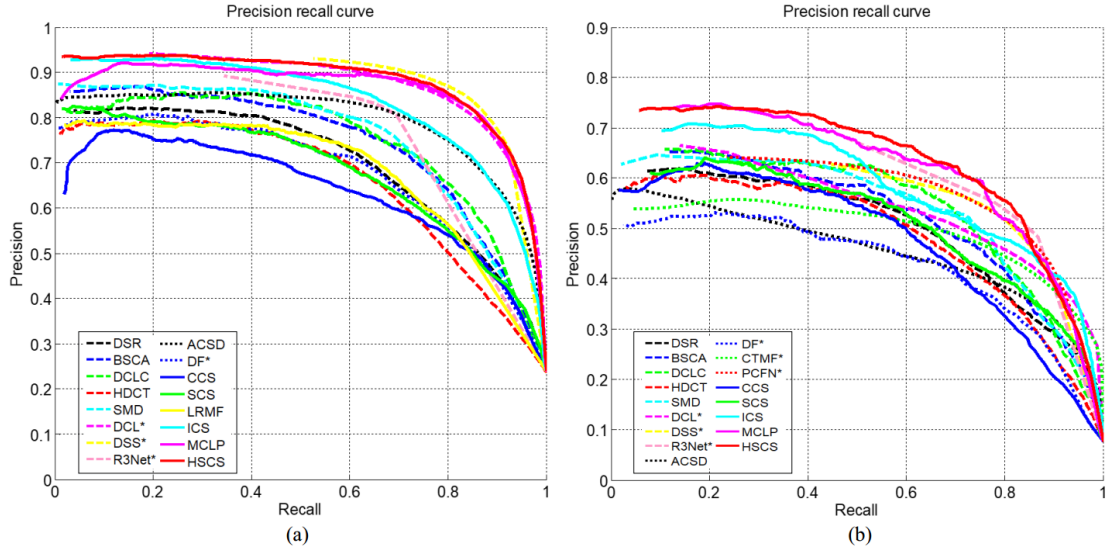
Fig. 6-4 PR curves of different methods on two RGBD co-saliency detection datasets, where “*” denotes the deep learning based methods. (a) PR curves on the RGBD Cosal150 dataset. (b) PR curves on the RGBD Coseg183 dataset.
