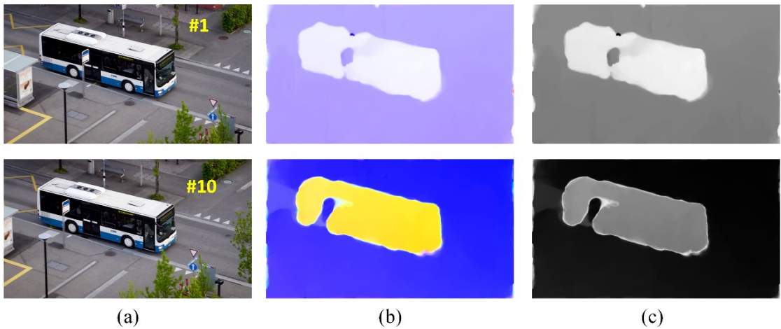
Fig. 7-2 Optical flow data of different video frames. (a) RGB image. (b) Optical flow map. (c) The MOF data.
