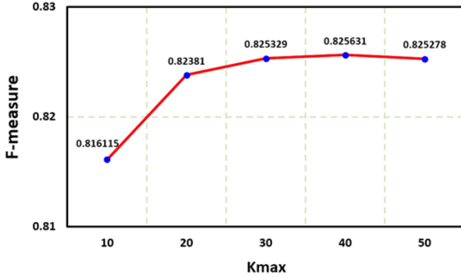
Fig. 4-4 F-measure of inter saliency map on the RGBD Cosal150 dataset under different maximum matching numbers.
