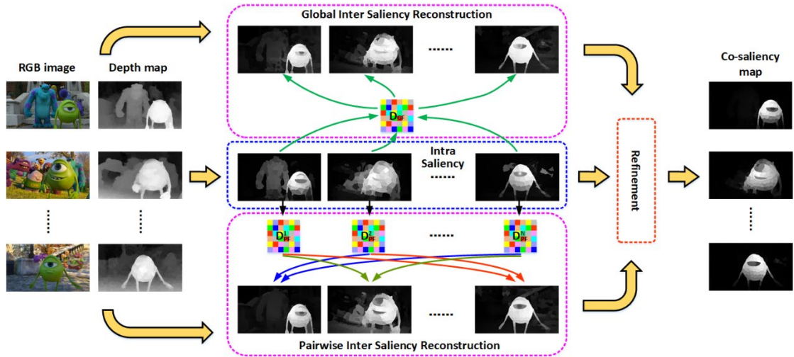
Fig. 6-1 Flowchart of the proposed RGBD co-saliency detection method.
