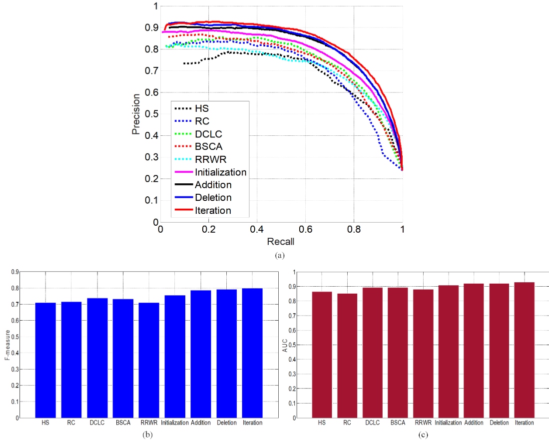
Fig. 5-8 Quantitative comparisons of the each part of the proposed framework on RGBD Cosal150 dataset. (a) PR curves. (b) F-measure. (c) AUC score.
