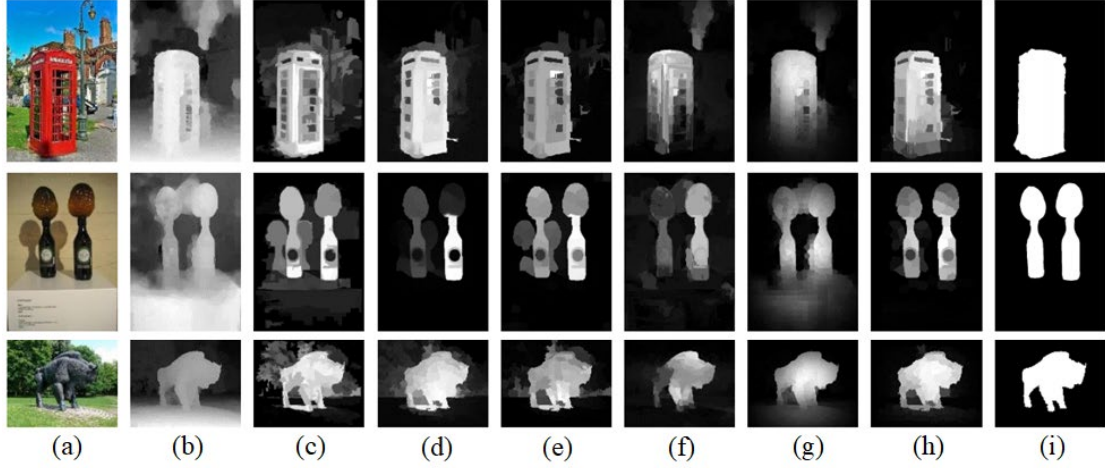
Fig. 3-5 Visual comparisons of saliency maps. (a) Input RGB image. (b) Input depth map. (c) RC. (d) RRWR. (e) DCLC. (f) SS. (g) ACSD. (h) Ours. (i) Ground truth.
