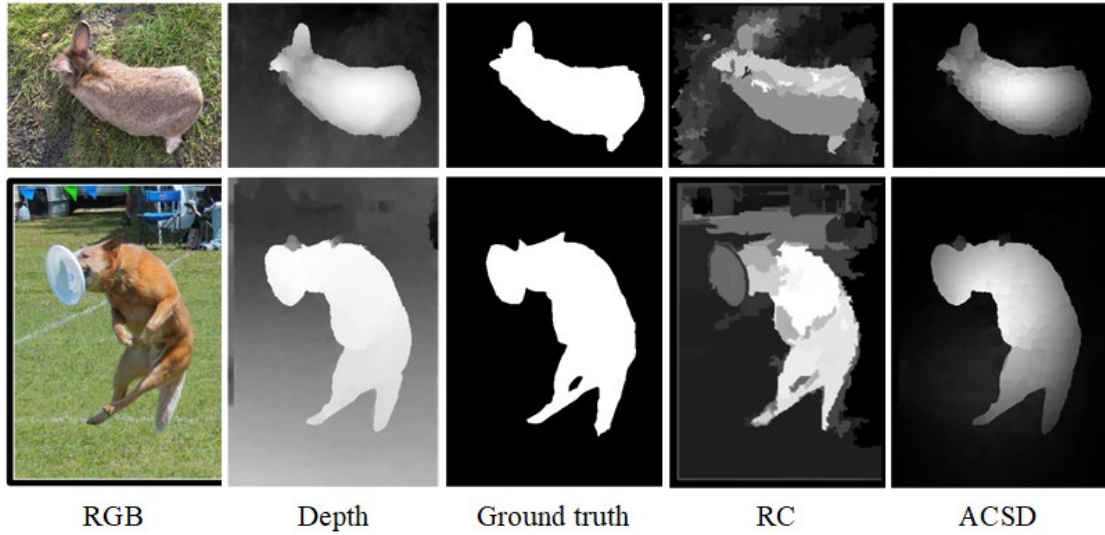
Fig. 1-1 Some illustrations of saliency detection with and without depth cue. The first three columns correspond to the RGB image, depth map, and ground truth, respectively. The fourth column shows the image saliency detection result using the RC method [25]. The fifth column represents the RGBD saliency detection result using the ACSD method [65].
