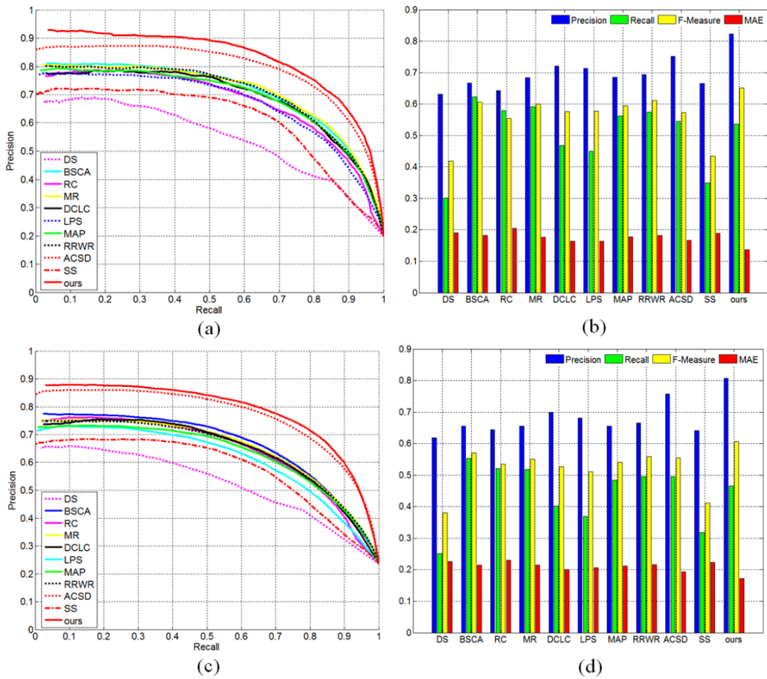
Fig. 3-4 Quantitative comparisons of proposed method with 10 state-of-the-art methods. (a) PR curves of different methods on NJU-400 dataset. (b) Average precision, recall, F-measure, and MAE of different methods on NJU-400 dataset. (c) PR curves of different methods on NJUD dataset. (d) Average precision, recall, F-measure, and MAE of different methods on NJUD dataset.
