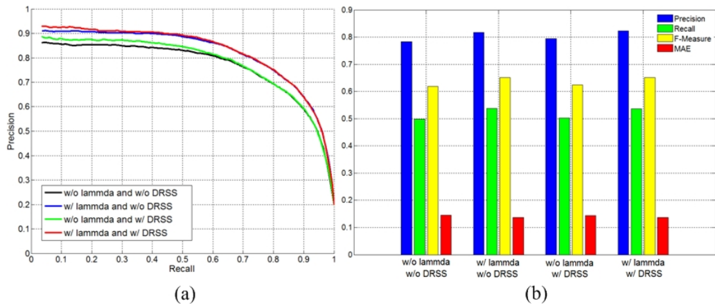
Fig. 3-6 Evaluation of different factors on NJU-400 dataset. (a) PR curves of different factors. (b) Average precision, recall, F-measure, and MAE score of different factors.
