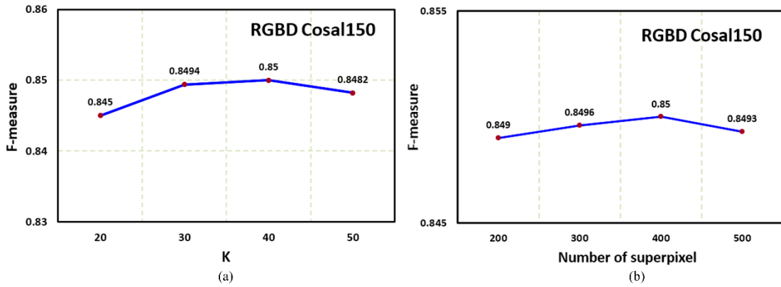
Fig. 6-5 F-measure of different parameters on the RGBD Cosal150 dataset. (a) The influence of different number of initial foreground seeds. (b) The influence of different number of superpixels.
