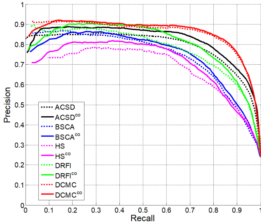
Fig. 4-6 PR curves of co-saliency results on the RGBD Cosal150 dataset with different intra saliency maps. The subscript of “co” means the co-saliency result produced by the proposed co-saliency model with the CLP optimization and corresponding intra saliency initialization.
