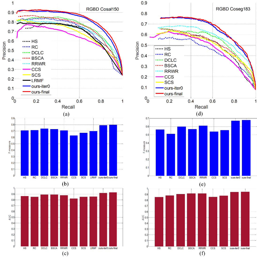
Fig. 5-7 Quantitative comparisons between the proposed method and the state-of-the-art methods on two datasets. Notice that “ours-iter0” means the co-saliency without iteration scheme, and “ours-final” denotes the co-saliency result with iteration scheme. (a)-(c) PR curves, F-measure, and AUC scores on the RGBD Cosal150 dataset. (d)-(f) PR curves, F-measure, and AUC scores on the RGBD Coseg183 dataset.
