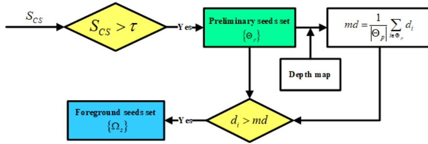
Fig. 3-3 Flowchart of depth-refined foreground seeds selection mechanism.
