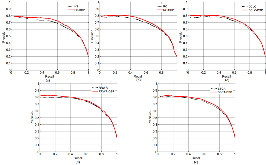
Fig. 5-10 Quantitative evaluation of the DSP on NJU-400 dataset. The black line in each PR curve denotes the original RGB saliency result, and the red line represents the saliency result with depth shape prior. The PR curves for (a) HS, (b) RC, (c) DCLC, (d) RRWR, and (e) BSCA methods.
