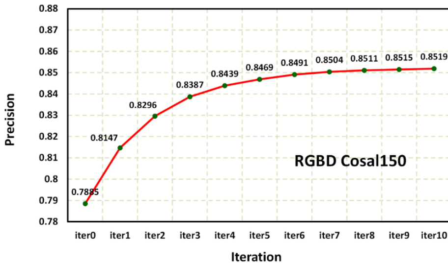
Fig. 5-9 Average precision of each iteration on the RGBD Cosal150 dataset.
