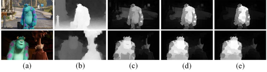
Fig. 5-2 Some examples of the proposed method. (a) RGB image. (b) Depth map. (c) The initialized saliency map. (d) The co-saliency map without iteration. (e) The final co-saliency map with iteration.
