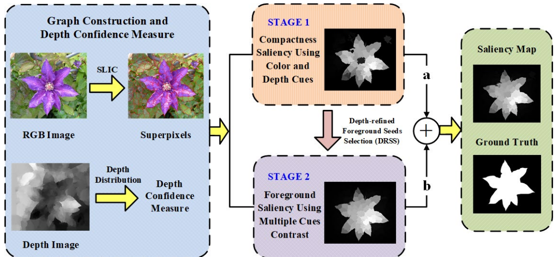
Fig. 3-1 Flowchart of the proposed method.
