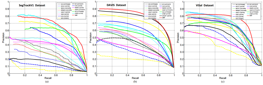
Fig. 7-4 PR curves of different methods on three datasets. (a) SegTrackV1 dataset. (b) DAVIS dataset. (c) ViSal dataset.
