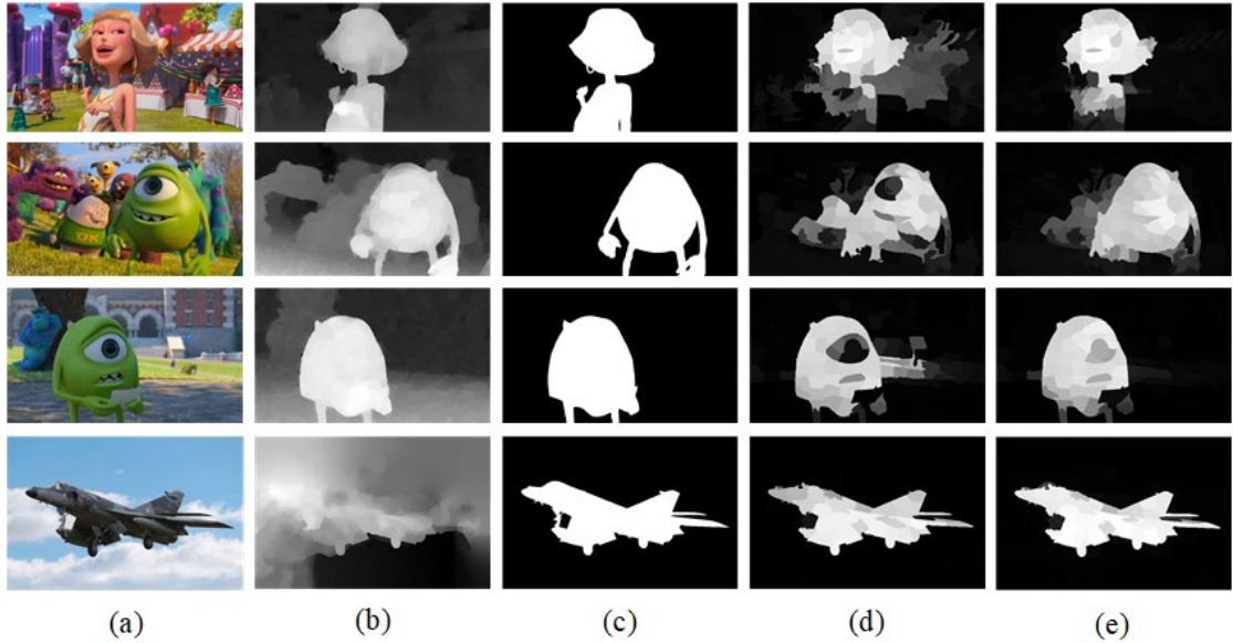
Fig. 4-5 Visual examples with and without depth information through the proposed co-saliency detection method. (a) RGB images. (b) Depth maps. (c) Ground truth. (d) Saliency maps without depth information. (e) Saliency maps with depth information.
