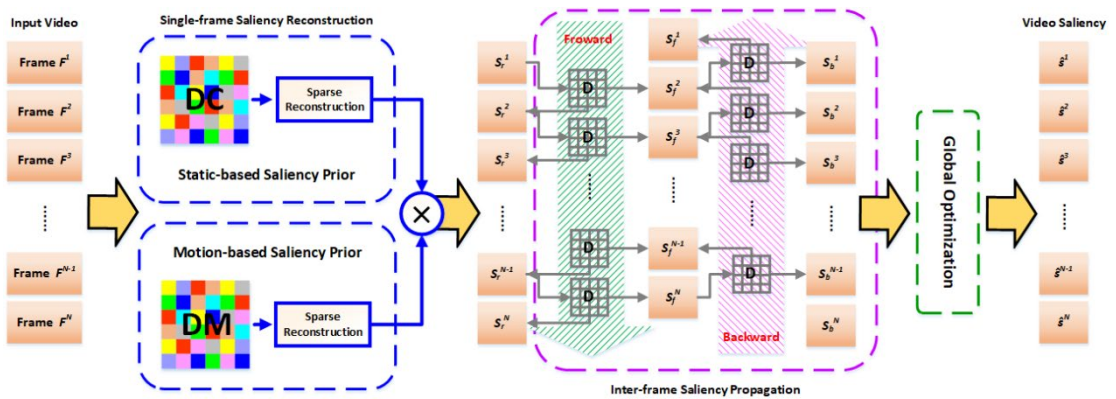
Fig. 7-1 Flowchart of the proposed video saliency detection framework.
