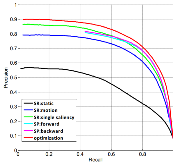
Fig. 7-5 PR curves of different modules of the proposed method on the DAVIS dataset.
