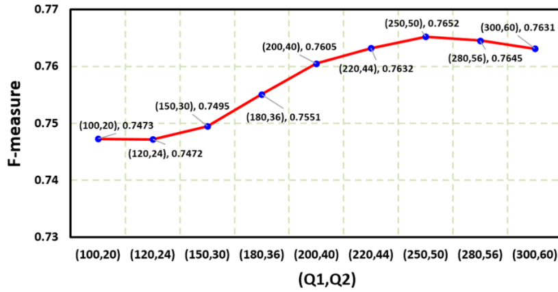
Fig. 7-6 F-measure of different (Q_1, Q_2) on the DAVIS dataset.
