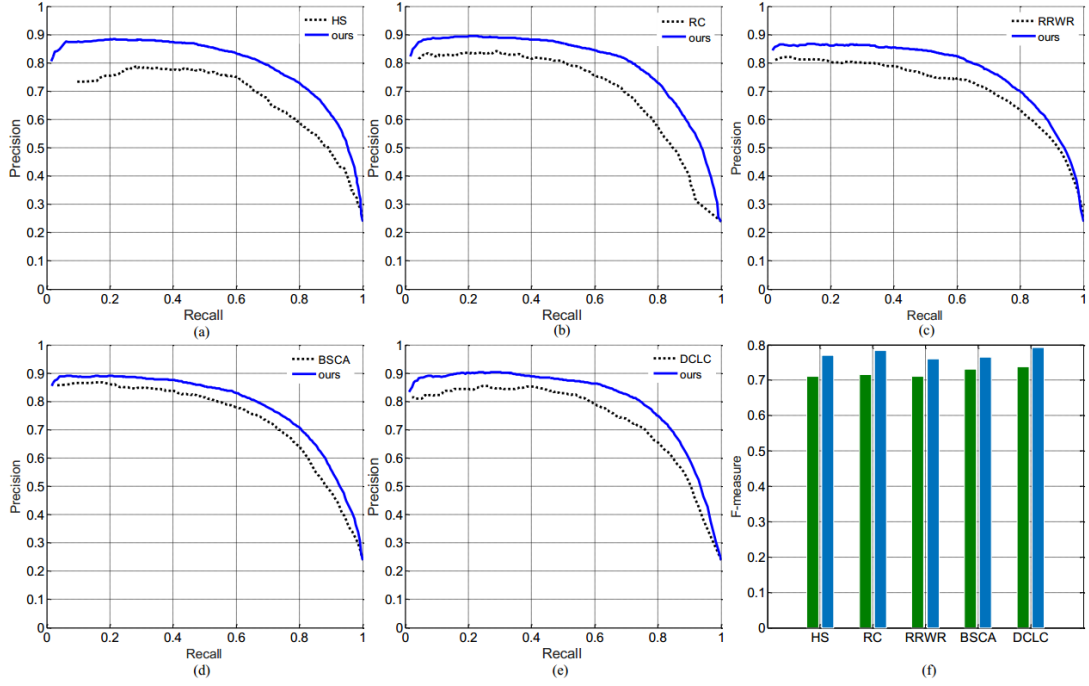
Fig. 5-11 Quantitative evaluation of one-for-one option for the proposed framework on the RGBD Cosal150 dataset. The black line in each PR curve denotes the original RGB saliency result, and the blue line represents the final co-saliency result using the proposed framework. The PR curves with different input saliency maps, i.e. , (a) HS, (b) RC, (c) RRWR, (d) BSCA, and (e) DCLC. (f) F-measure of the one-for-one framework.
