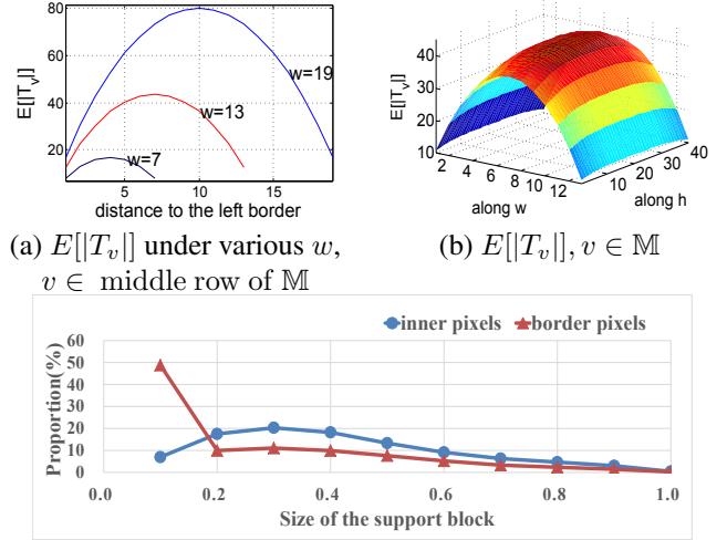
Fig. 3. Mathematical and statistical results of the toy example.
