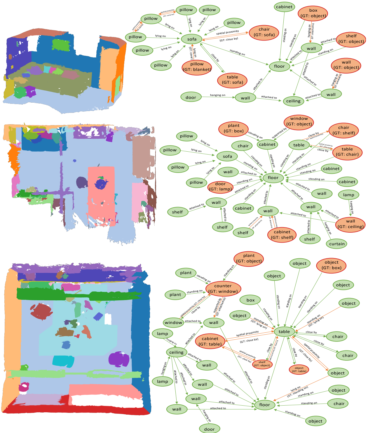
Figure 1. Qualitative visualization of the SGG point framework, where misclassified object and structural relationship samples are marked with ground truth values in red, while the correct ones are shown in green with ground truth values omitted.
