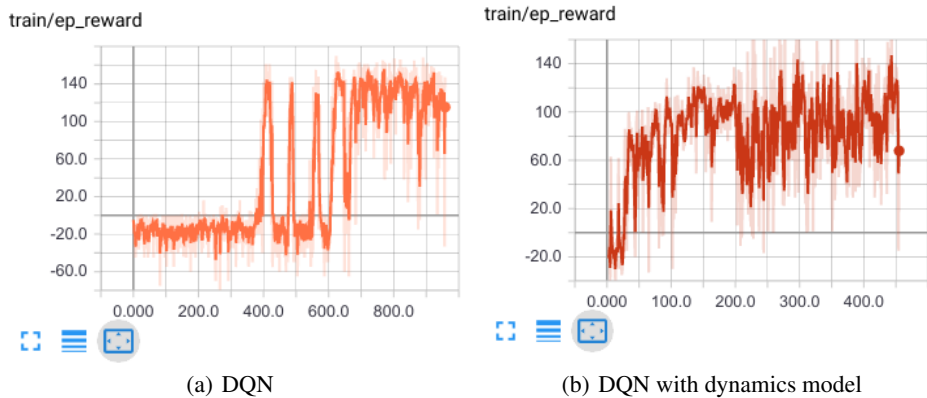
Figure 7: Average training rewards vs number of real episodes in Maze
