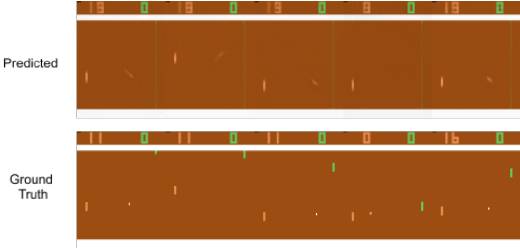
Figure 8: Prediction model on Pong
