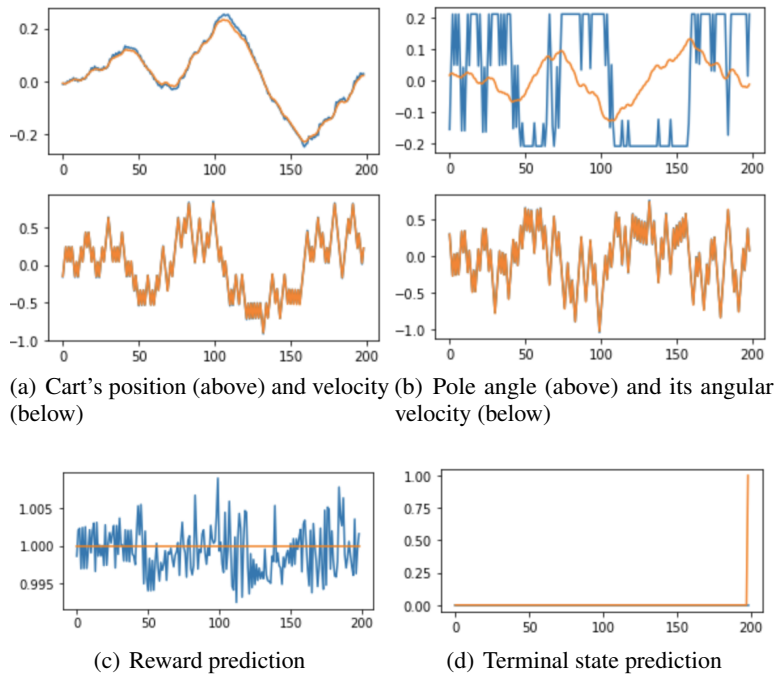
Figure 5: Predictions from model dynamics approximation
