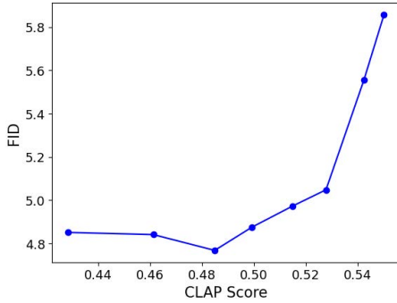
Figure 7. Classifier-free guidance trade-off curves.
