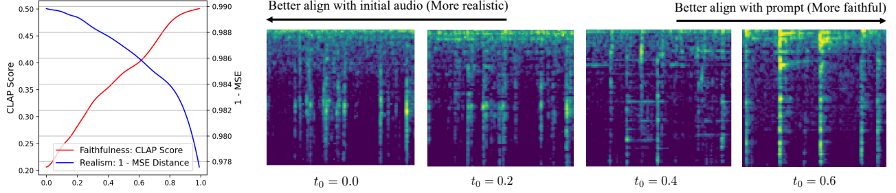
Figure 5. We illustrate personalized text-to-audio results with various t_0 initializations. t_0 = 0 indicates the initial audio itself, whereas t_0 = 1 indicates a text-to-audio synthesis from scratch. For comparison, realism is measured by the 1-MSE distance between generated and initial audio, and faithfulness is measured by the CLAP score between the generated sample. Prompt: A clock ticktocks.
