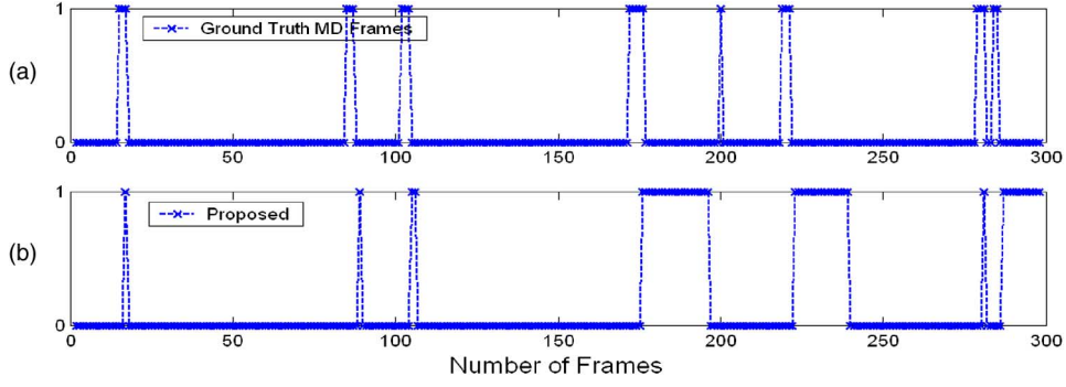
Fig. 11. Detection result of the proposed algorithm in Stefan_Sif .
