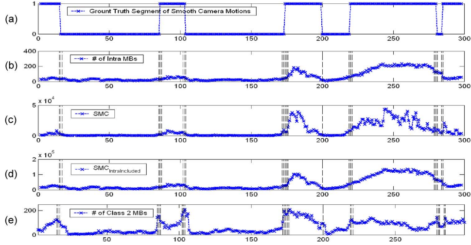
Fig. 10. Feature curves for the MD detection in Stefan_Sif .
