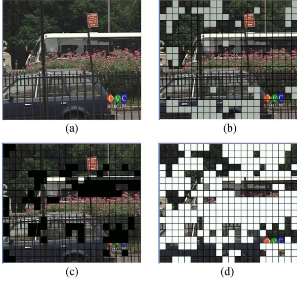
Fig. 2. (a) Original frames and the distributions of (b) Class 1, (c) Class 2, and (d) Class 3 MBs for Mobile_Cif using (2).
