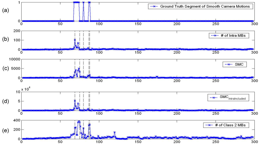
Fig. 12. Feature curves for the MD detection in Coastguard_Cif .
