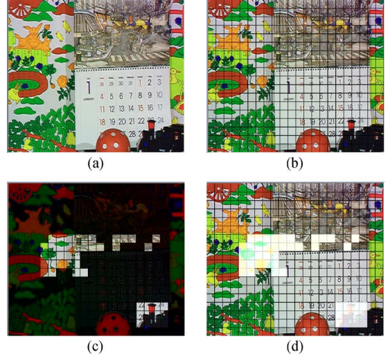
Fig. 4. MB distributions at the abrupt shot change frame from Bus_Cif to Mobile_Cif . (a) Original frame. (b) Class 1. (c) Class 2. (d) Class 3.
