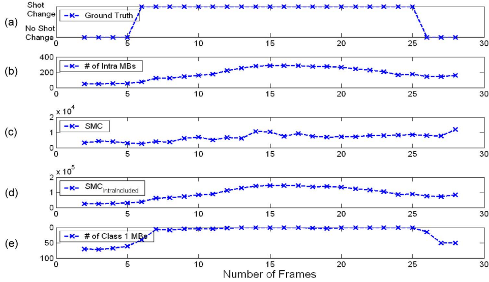
Fig. 8. Feature curves of a gradual shot change sequence.
