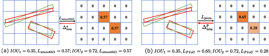
Fig. 1. Comparison between PIoU and SmoothL1 [34] losses. (a) Loss values between IoU and SmoothL1 are totally different while their SmoothL1 loss values are the same. (b) The proposed PIoU loss is consistent and correlated with IoU.
