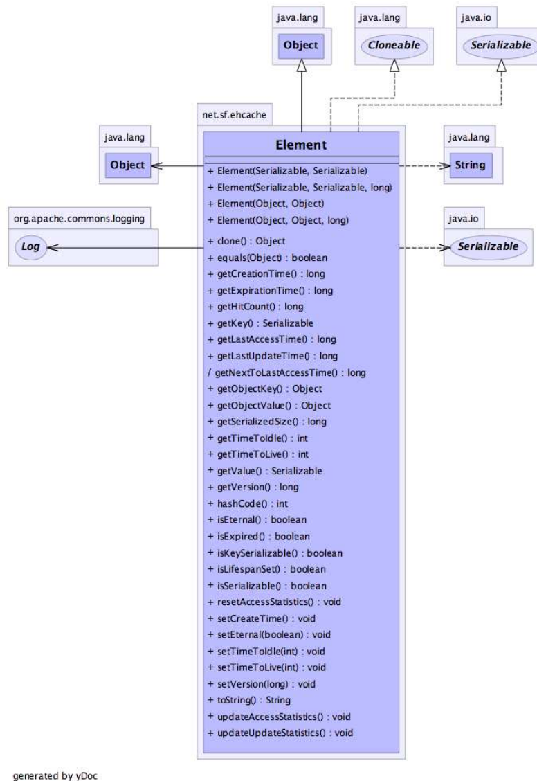
Element Class Diagram
