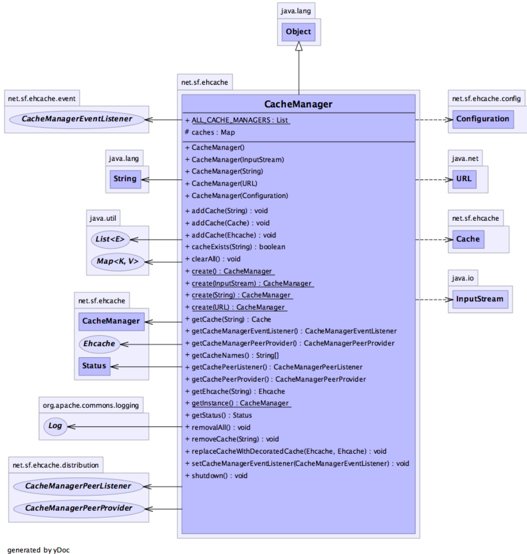
CacheManager Class Diagram
