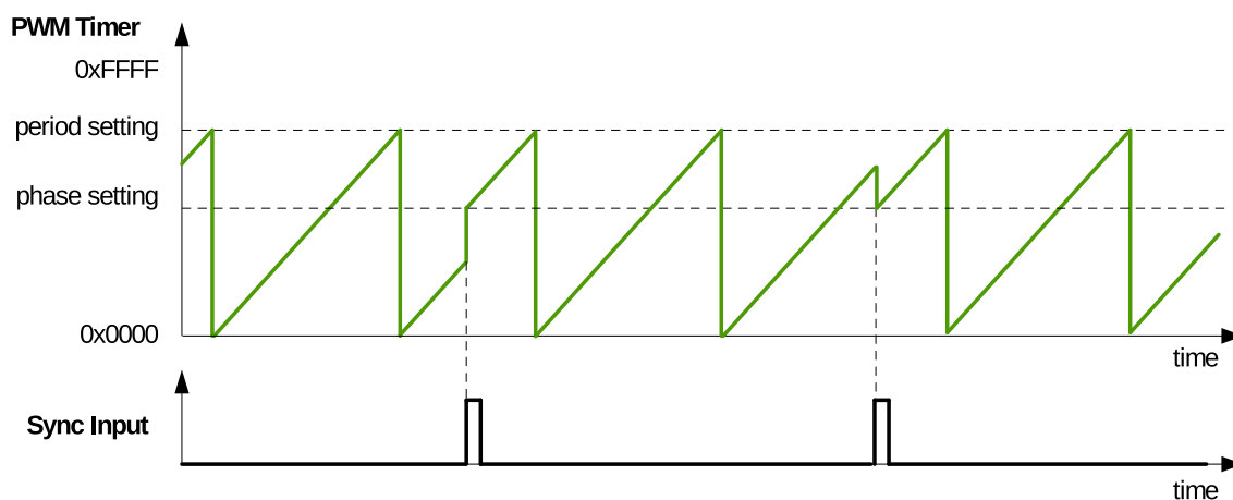
Figure 29.3-6. Count-Up Mode Waveform
