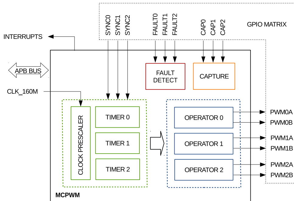
Figure 29.2-1. MCPWM Module Overview
