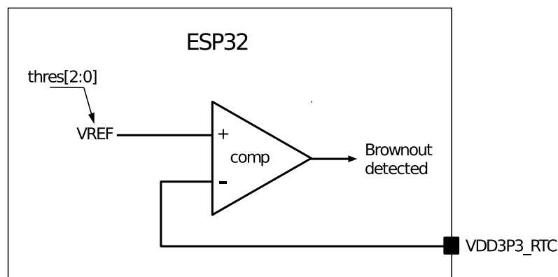
Figure 9.3-4. Brownout Detector
