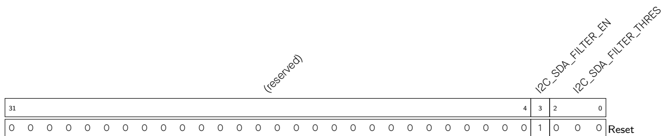
Register 21.20. I2C_SDA_FILTER_CFG_REG (0x0054)
