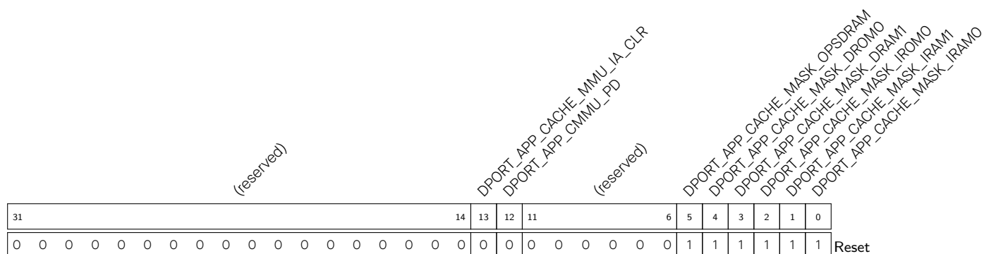
Register 12.13. DPORT_APP_CACHE_CTRL1_REG (0x05C)
