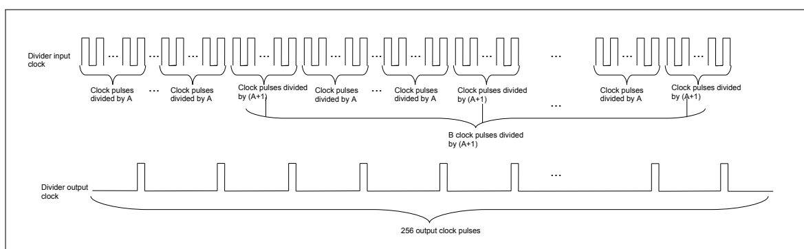
Figure 28.2-3. LED_PWM Divider
