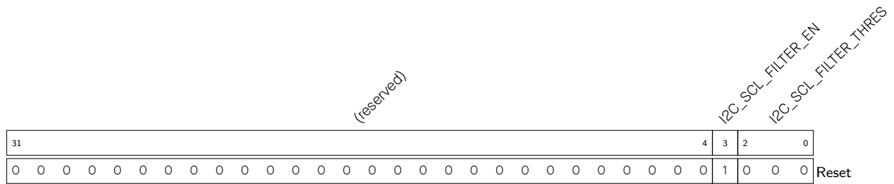
Register 21.19. I2C_SCL_FILTER_CFG_REG (0x0050)
