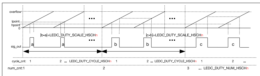
Figure 28.2-5. Output Signal Diagram of Fading Duty Cycle
