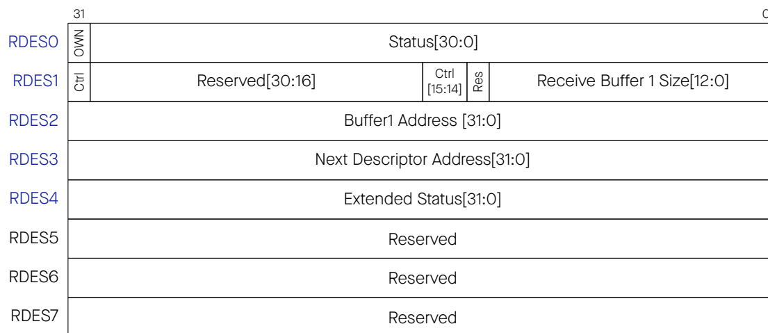
Figure 24.8-2. Receive Descriptor
