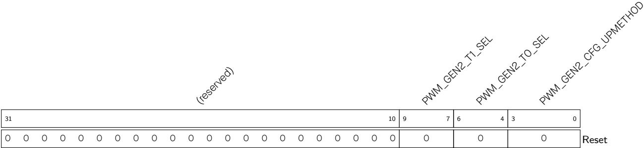
Register 29.47. PWM_GEN2_CFG0_REG (0x00b8)
