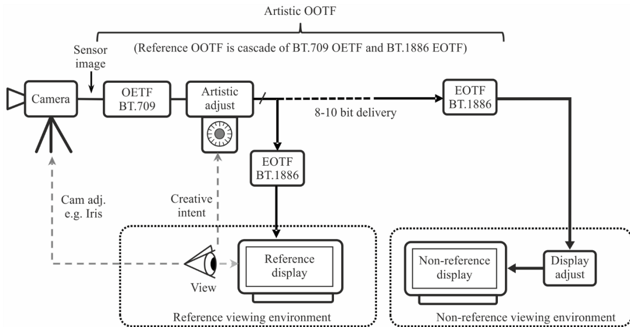
FIGURE 10 The BT.709 HDTV television system architecture
