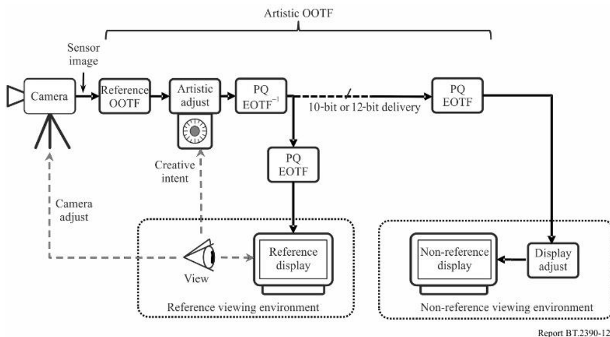
FIGURE 12 PQ HDR-TV system with 10-bit or 12-bit integer values
