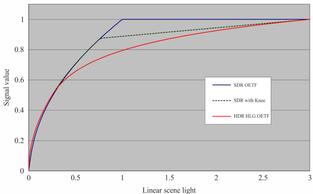
FIGURE 18 Comparison of SDR and HLG HDR OETFs
