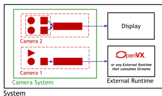
Figure 2. An example Camera System with Devices, Streams and Cameras
