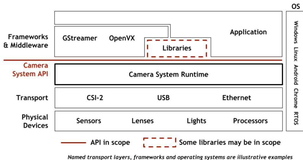
Figure 1. Camera System Runtime and API with optional Libraries
