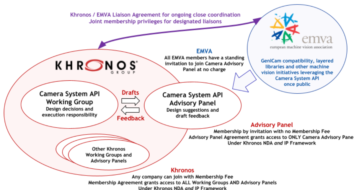
Figure 3. Proposed Camera System API coordination between EMVA and Khronos
