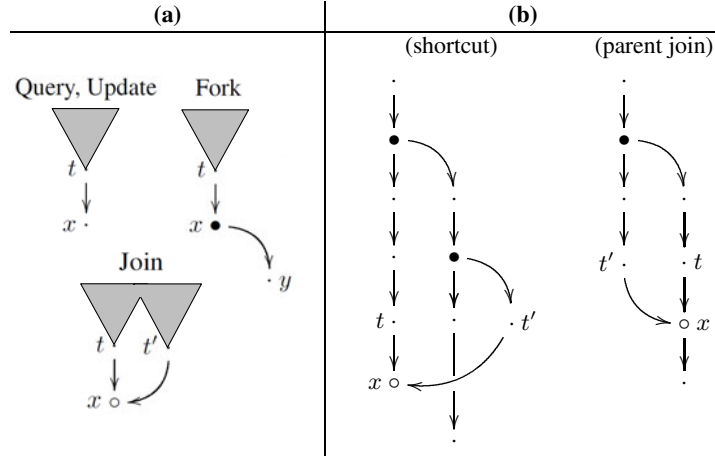
Fig. 2. (a) (left) Visualization of the construction rules for revision diagrams in Def. 6. (b) (right) Examples of invalid revision diagrams. Both diagrams are not possible since they violate the join property at the creation of the join node x . Note that in the right diagram, F(t') is undefined on the main revision and therefore F(t') \rightarrow^* t does not hold.
