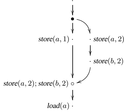
Fig. 3. A labeled revision diagram. The path-result of the bottom vertex is now the query applied to its root-path: \text{load}(a)^\#(\text{store}(b, 2)^\#(\text{store}(a, 2)^\#(\text{store}(a, 1)^\#(s_0)))) = 2 .
