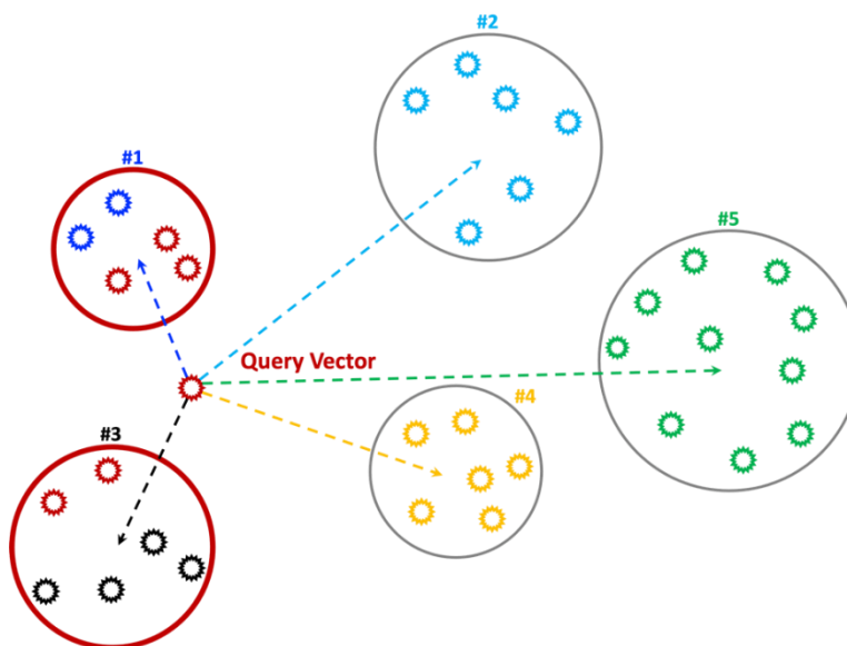
Figure 6: 2-Dimensional Data-Set
