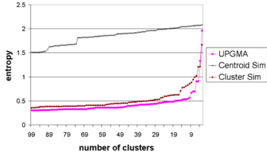
Figure 6: fbis entropy
