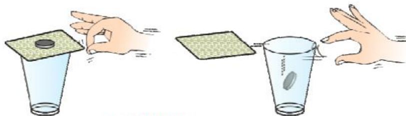
Law of Intertia
