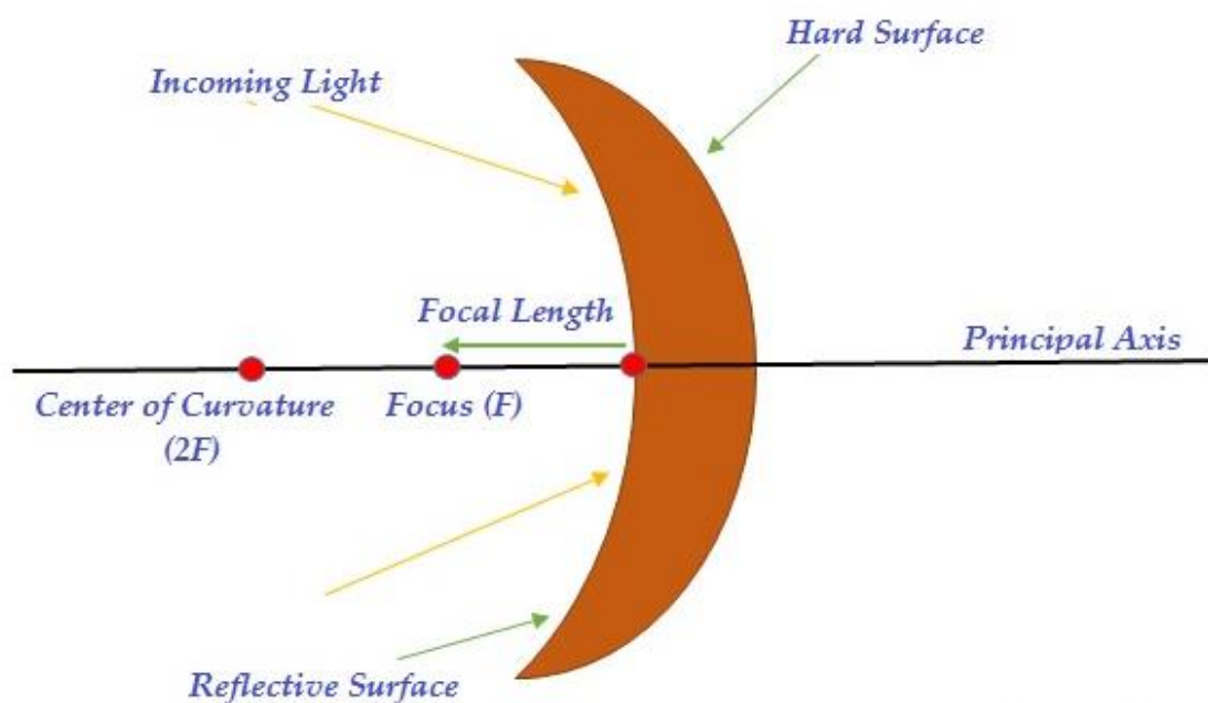
Concave Mirror Diagram
