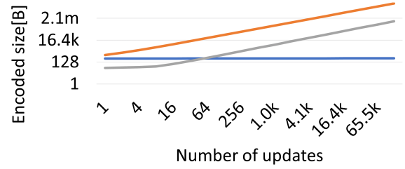
(b) Map size when inserting and removing a map key.
