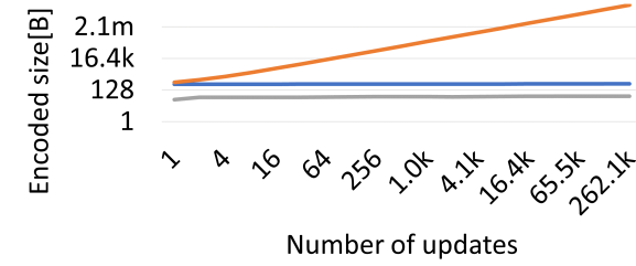
(a) Map size when updating the same key in a map.
