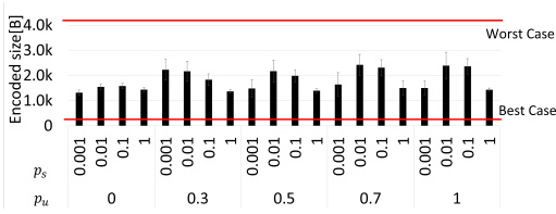
Figure 5: Document size for 5 replicas, where each replica either performs an update with probability p_u , sorts with probability 1 - p_u , and synchronizes with probability p_s .
