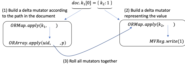
Figure 2: Transform a JavaScript operation doc.k_1[0] = \{k_2: 1\} to a delta mutation in the JSON CRDT, where p = \text{GETPosFromIdx}(0) and uid = \text{GETUidFromIdx}(0) .
