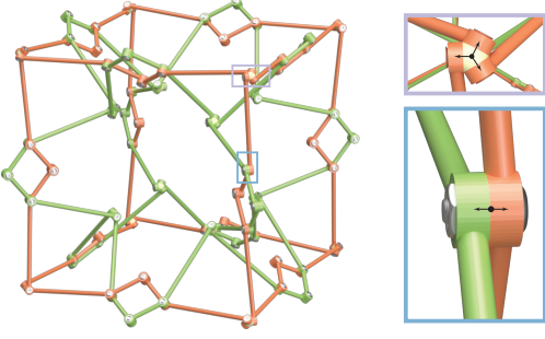
Figure 11: To construct a mechanically sound linkage, the positions of the bars' endpoints are offset from the joint centers (inset). These offsets need to be considered to avoid collisions.
