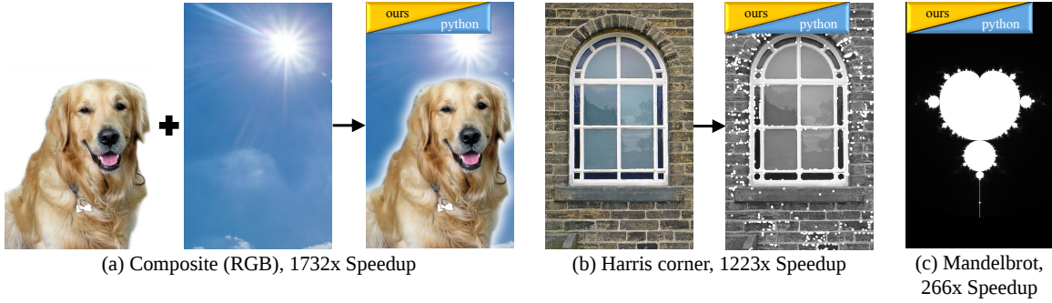
Figure 1: Three applications that were compiled with our compiler, which is specialized for visual computing programs. Image compositing (a) gains a 1732 \times speedup over the equivalent code in the Python interpreter. Our result is shown in the diagonal upper-left corner; and the Python result is shown in the diagonal lower-right corner: notice there is no difference between the two images. A Harris corner detector (b) and a Mandelbrot fractal renderer (c) likewise gain significant speedups after being compiled with our compiler, relative to Python. Photo credits: (a) Karen Arnold and Skitterphoto, (b) modified from original by Tim Green.
