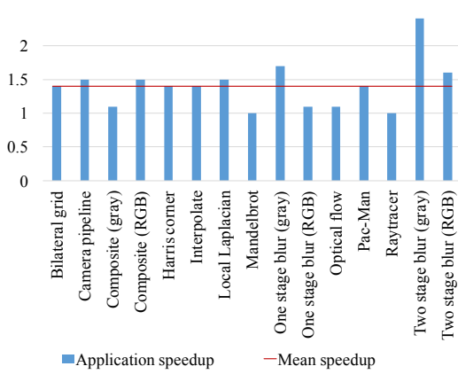
Figure 6: The speedup of the 32-bit floating-point variant of each application relative to the 64-bit variant.
