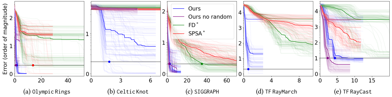
Fig. 8. Runtime-Error plot for five optimization tasks, comparing Ours (with and without random variables) with FD* and SPSA* – using 100 restarts with random initialization and plot axes as in Figure 7. Note we select FD* and SPSA* based on minimal error from among 10 and 30 different variants, as discussed in Section 8.2. Grey horizontal lines denote success threshold, while circles on grey lines mark median success time as in Table 4.
